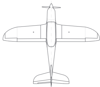
wing span 7.9m, wing area 9.5 m 2
